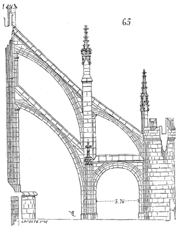
arcs-boutants
